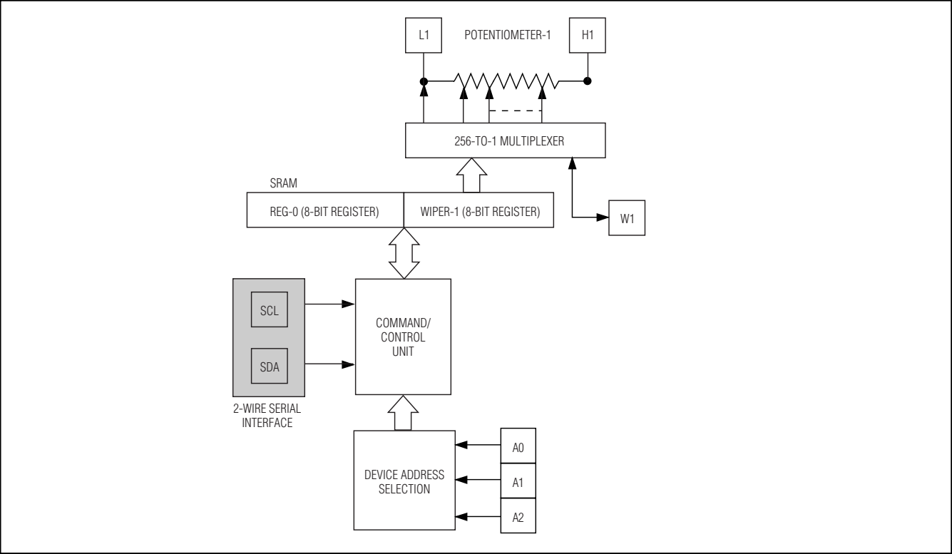
Figure 1. Functional Diagram
