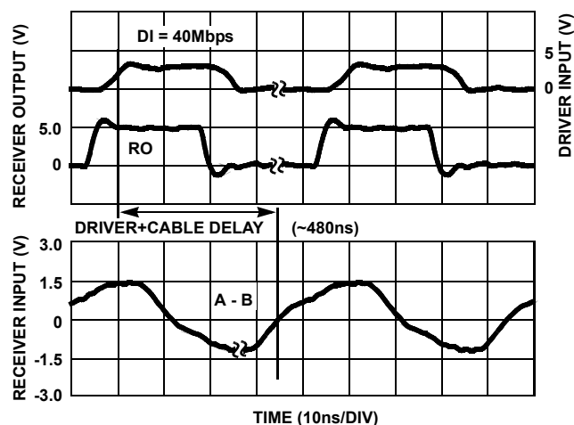
FIGURE 18. DRIVER AND RECEIVER WAVEFORMS DRIVING 350 FEET (107 METERS) OF CAT5 CABLE (DOUBLE TERMINATED WITH 120\Omega )
