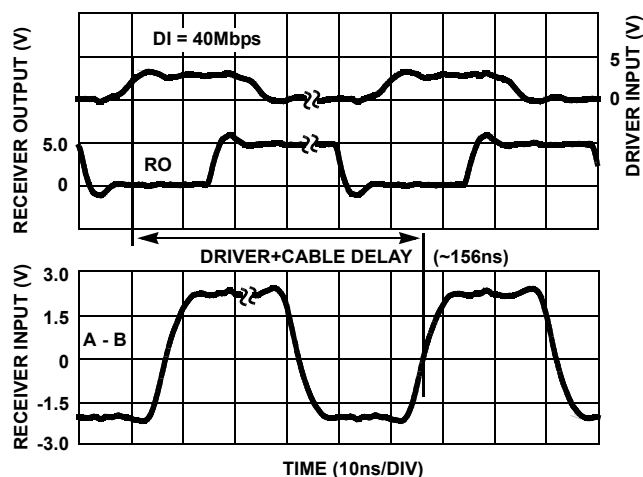
FIGURE 17. DRIVER AND RECEIVER WAVEFORMS DRIVING 100 FEET (31 METERS) OF CAT5 CABLE (DOUBLE TERMINATED WITH 120\Omega )
