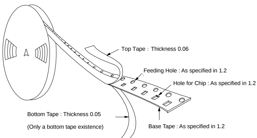
Fig.3 Taping Diagram
