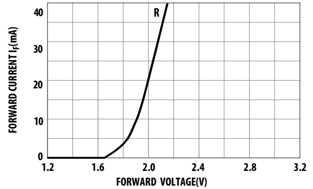
Figure 4. Forward Current vs. Forward Voltage
