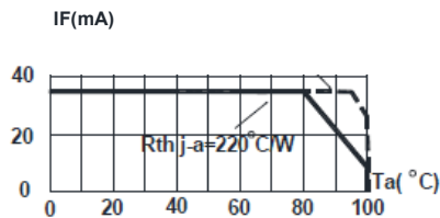
FIG.5 MAXIMUM FORWARD DC CURRENT VS AMBIENT TEMPERATURE ( T_{jmax}=110^{\circ}C )
