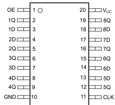
Figure 4-4. SN74AHCT374 PW, DW, N, DB, DGS Package (Top View)
