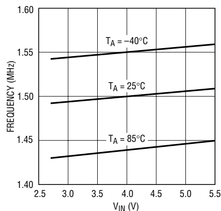
Oscillator Frequency vs Input Supply Voltage
