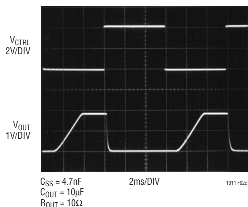
Figure 2. Shutdown/Soft-Start Operation
