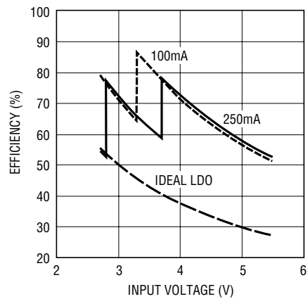
LTC1911-1.5 Efficiency vs Input Voltage (Falling Input Voltage)
