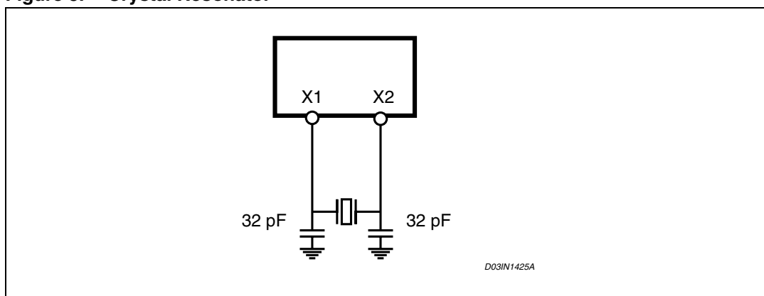
Figure 5. Crystal Resonator
