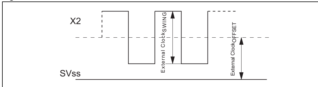
Figure 4. External clock waveform
