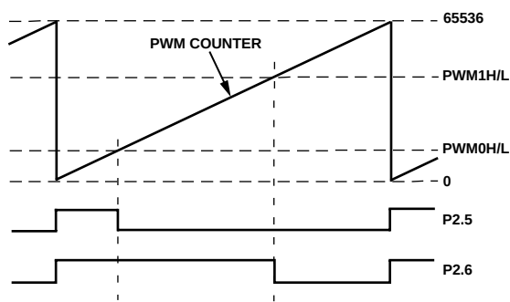
Figure 41. PWM Mode 3
