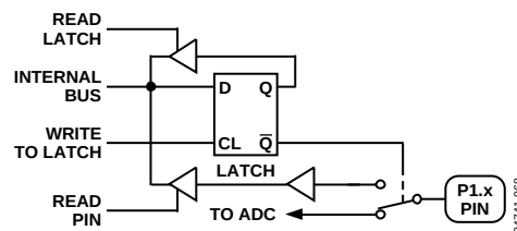
Figure 49. Port 1 Bit Latch and I/O Buffer
