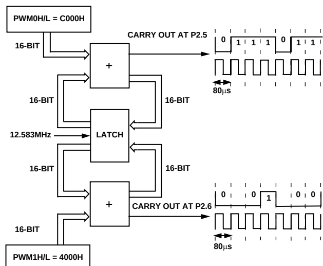
Figure 42. PWM Mode 4
