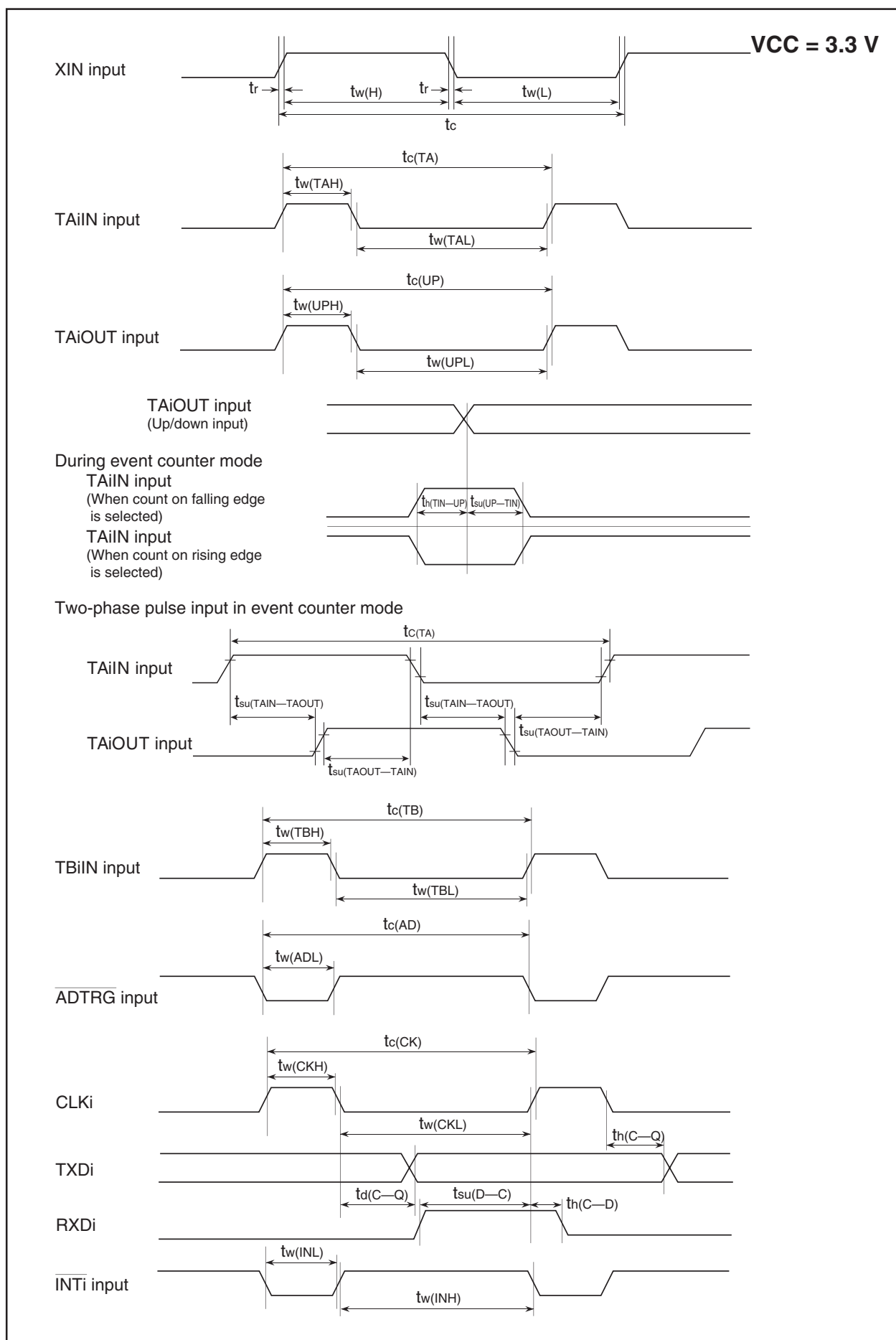
Figure 5.12 Timing Diagram (1)
