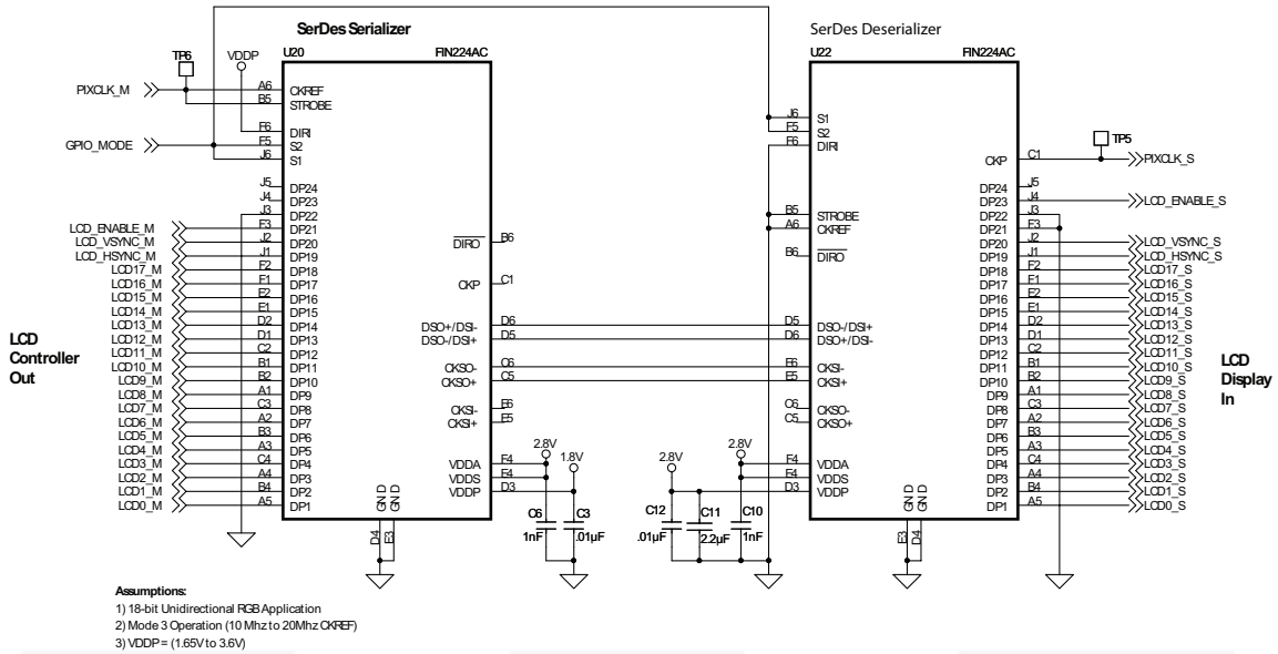
Figure 5. FIN224AC RGB
