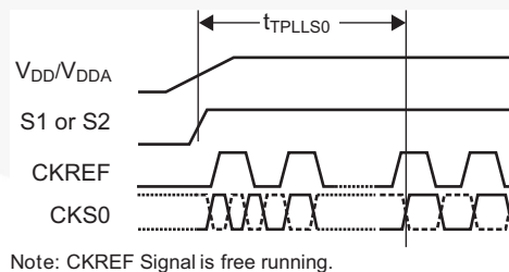
Figure 11. Serializer PLL Lock Time
