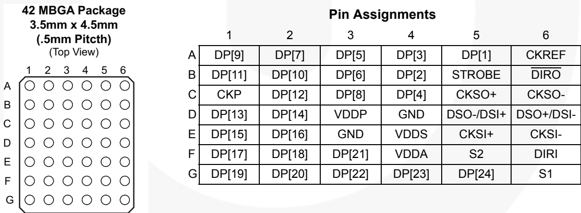
Figure 4. Terminal Assignments for \mu BGA (Top View)
