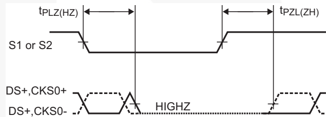
Figure 14. Serializer Enable and Disable Time
