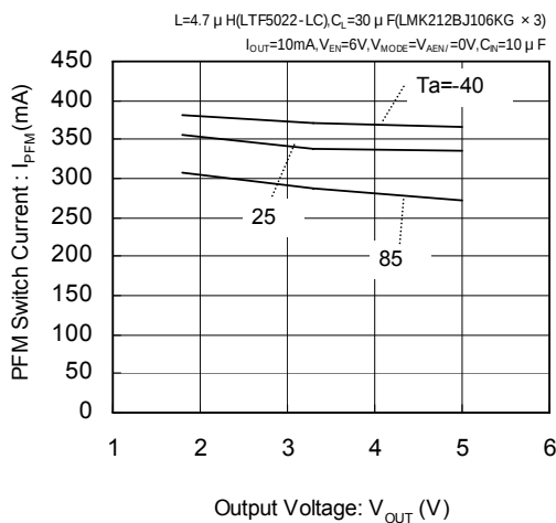
XC9128 ( V_{IN}=0.9V )
