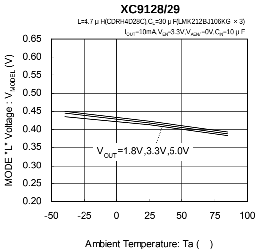
(37) MODE "L" Voltage vs. Ambient Temperature
