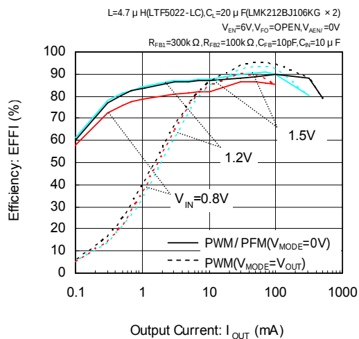
XC9128 ( V_{OUT}=1.8V )
