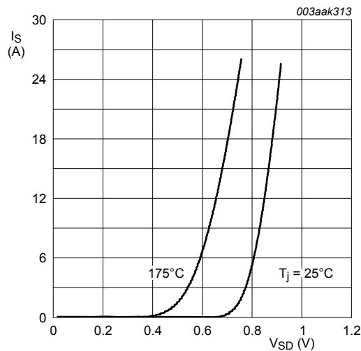
Fig. 16. Source (diode forward) current as a function of source-drain (diode forward) voltage; typical values V_{GS} = 0V
