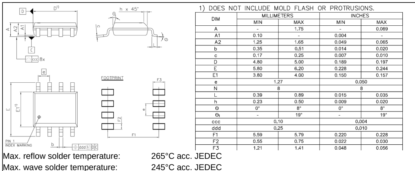
Figure 13 Package drawing
