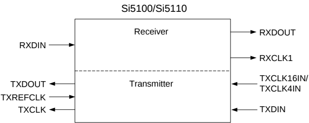
Figure 6. Full Duplex
