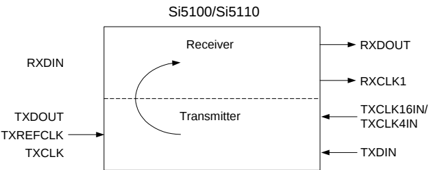
Figure 7. Diagnostic Loopback
