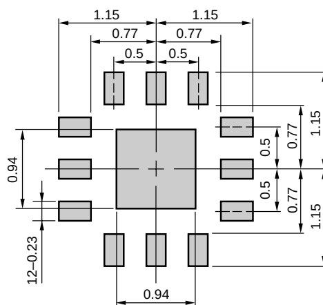
MOUNTING PAD
