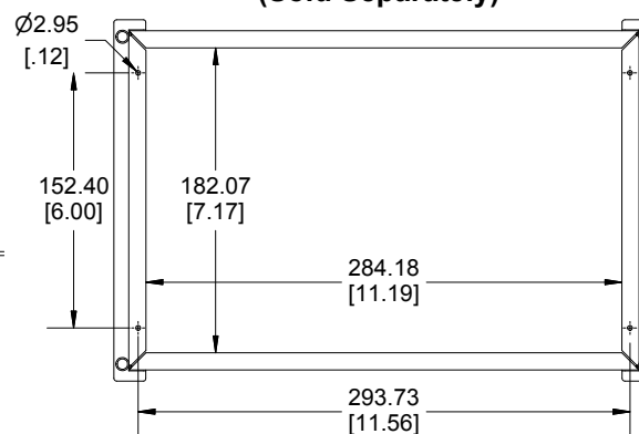
Bottom View of Chassis Assembly (Sold Separately)
