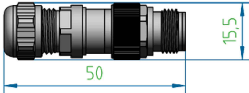
M12 D-4 MALE CABLE CLAMP RANGE FROM 4-6.5mm
