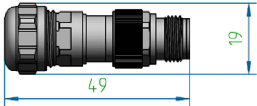
M12 D-4 MALE CABLE CLAMP RANGE FROM 5.5-9mm
