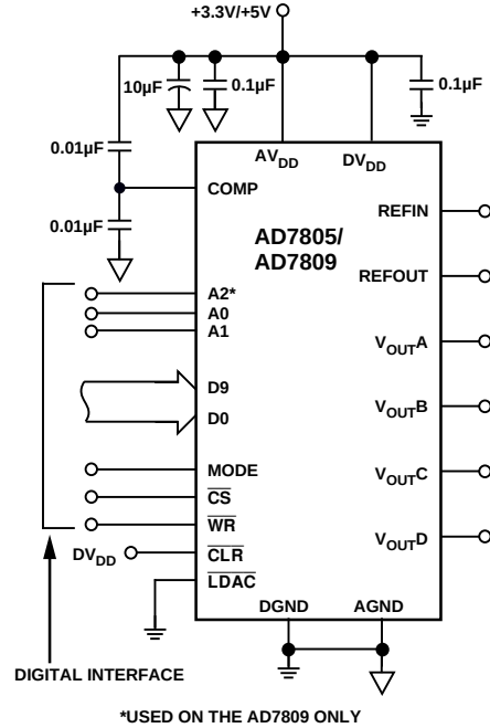
Figure 24. Typical Configuration for AD7805/AD7809
