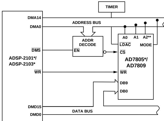
Figure 38. AD7805/AD7809–ADSP-2101/ADSP-2103 Interface
