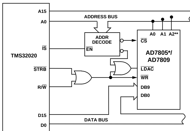
Figure 39. AD7805/AD7809–TMS32020 Interface
