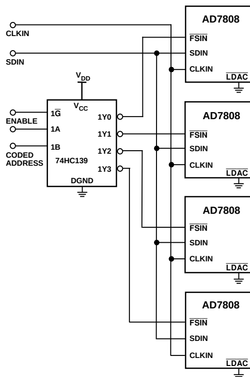
Figure 42. Decoding Multiple AD7808s Using the \overline{FSIN} Pin
