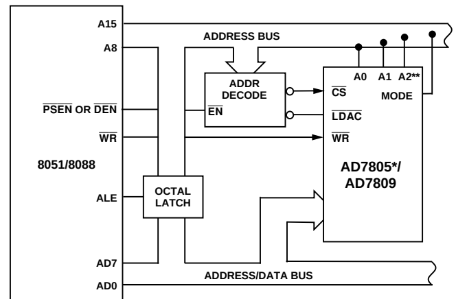
Figure 40. AD7805/AD7809–8051/8088 Interface
