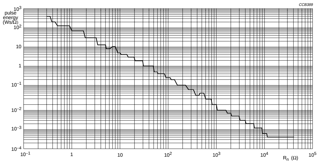
Fig.21 Pulse capability; W_s as a function of R_n .
