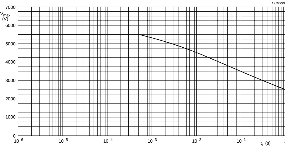
Fig.22 Pulse on a regular basis; maximum permissible peak pulse voltage ( \hat{V}_{max} ) as a function of pulse duration ( t_i ).
