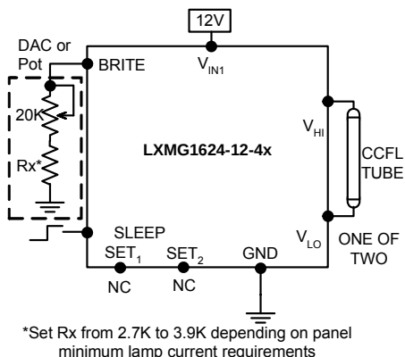
Figure 1 – Brightness Control (Output current set to maximum)
