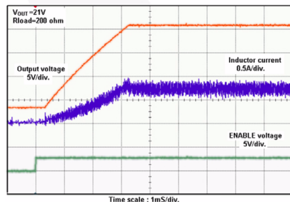
Figure 8. Start-up Response
