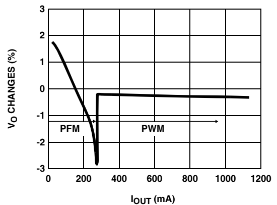
FIGURE 24. PFM-PWM LOAD REGULATION
