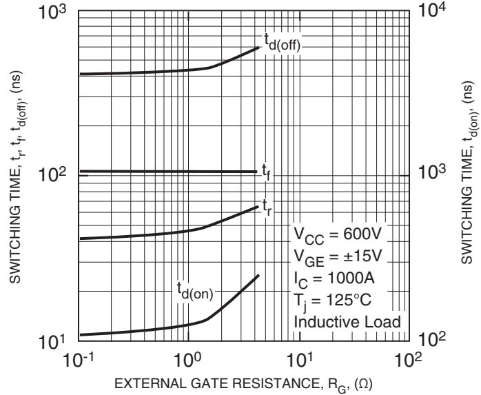
SWITCHING TIME VS. GATE RESISTANCE (TYPICAL)
