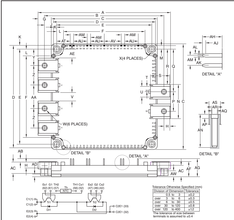
Outline Drawing and Circuit Diagram
