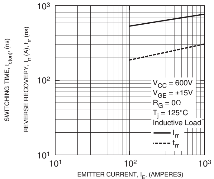
REVERSE RECOVERY CHARACTERISTICS (TYPICAL)
