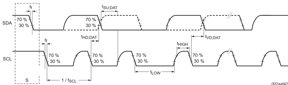
Fig 26. I 2 C-bus pins clock timing
