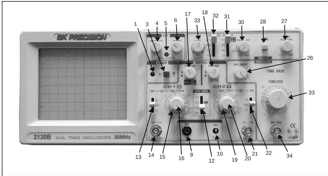
Fig. 2. Model 2120B Controls and Indicators.
