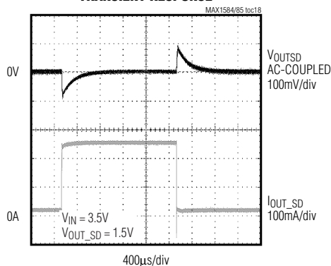
STEP-DOWN LOAD-TRANSIENT RESPONSE
