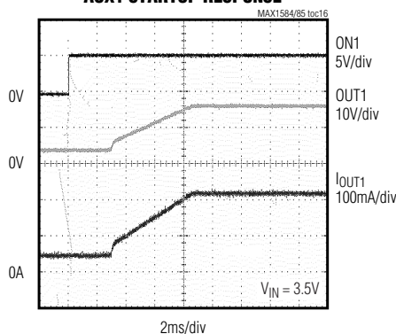
AUX1 STARTUP RESPONSE
