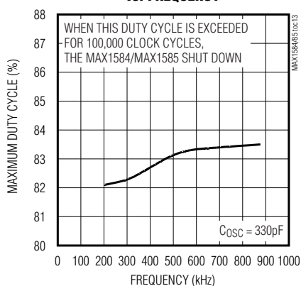
AUX MAXIMUM DUTY CYCLE vs. FREQUENCY
