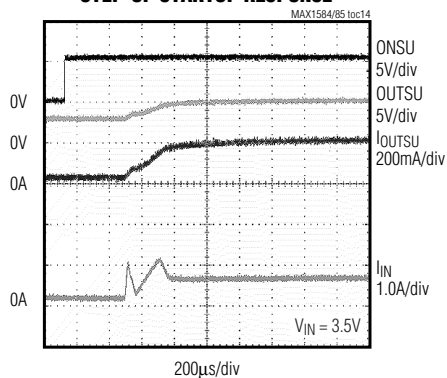
STEP-UP STARTUP RESPONSE
