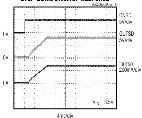
STEP-DOWN STARTUP RESPONSE
