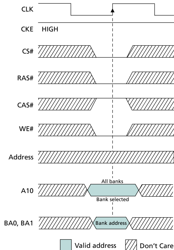
Figure 11: PRECHARGE Command
