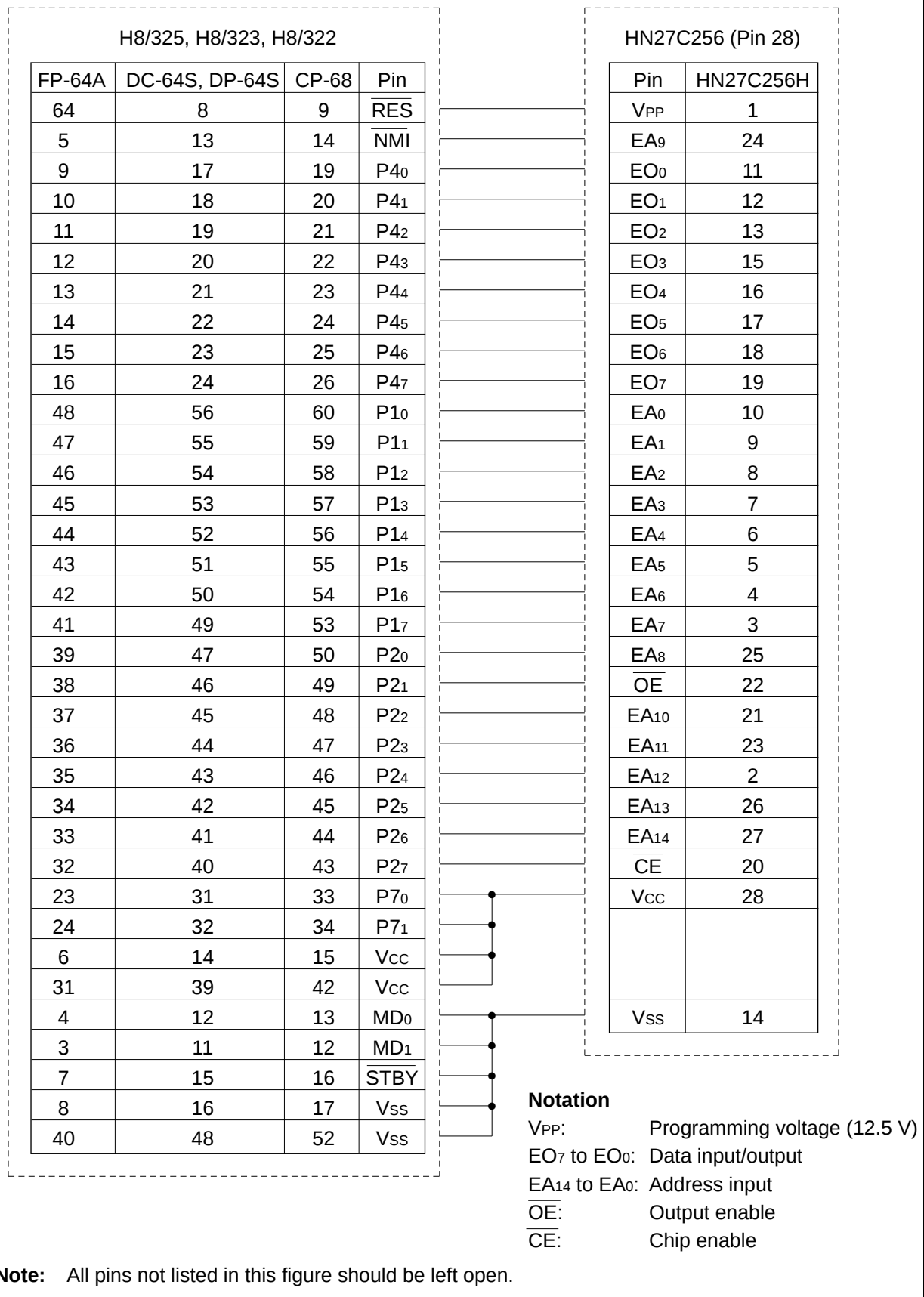
Figure 11-3. Socket Adapter Pin Assignments
