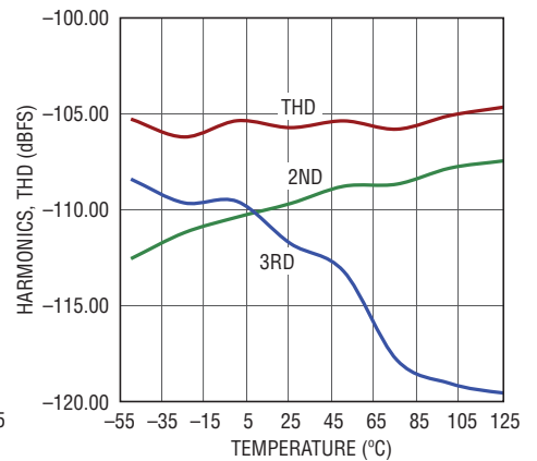
THD, Harmonics vs Temperature
