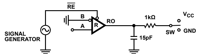
FIGURE 10. RECEIVER PROPAGATION DELAY AND DATA RATE
