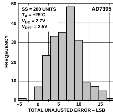
Figure 6. Total Unadjusted Error Histogram
