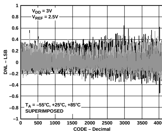
Figure 1. Differential Nonlinearity Error vs. Code
