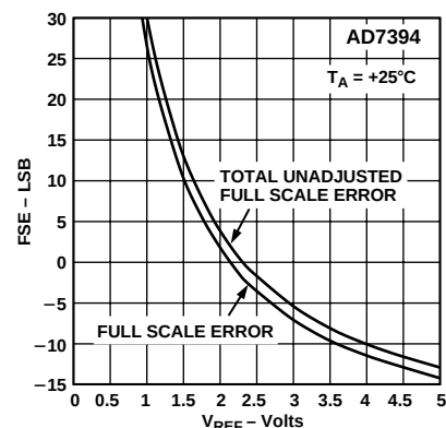
Figure 9. Full-Scale Error vs. V_{REF}
