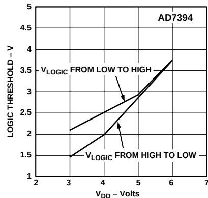
Figure 12. Logic Threshold vs. Supply Voltage
