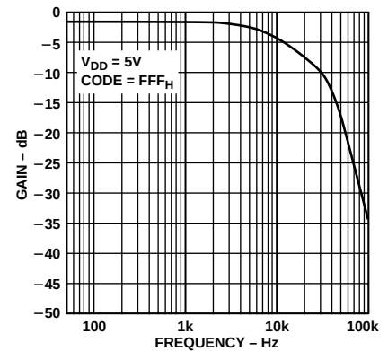
Figure 18. AD7395 Reference Multiplying Bandwidth
