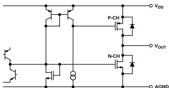
Figure 20. Equivalent Analog Output Circuit
