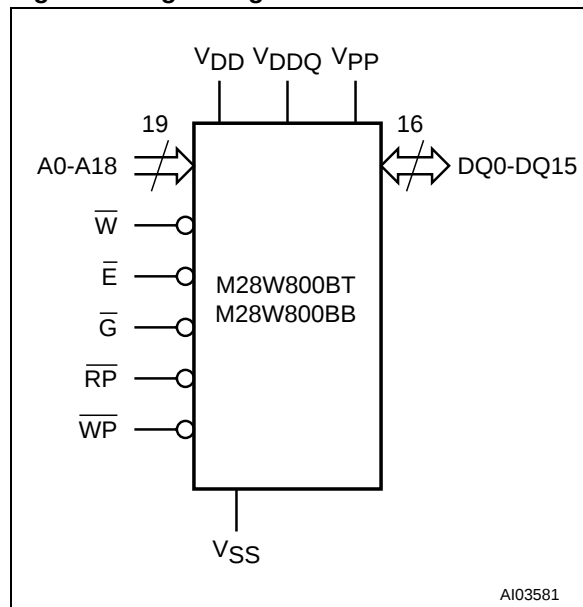
Figure 2. Logic Diagram
