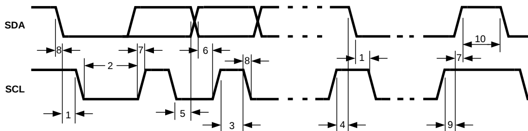
Figure 53. I²C Timing Diagram
