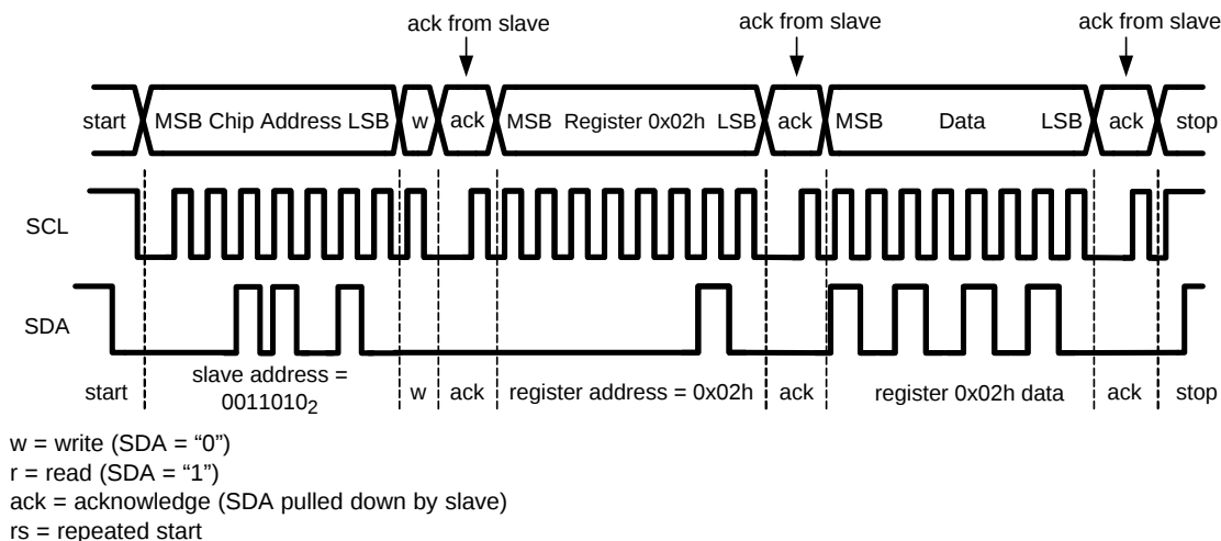
Figure 51. Example I²C Write Cycle
