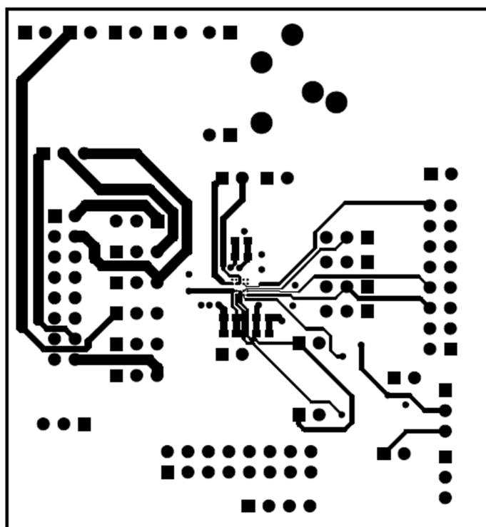
Figure 72. Bottom Layer
