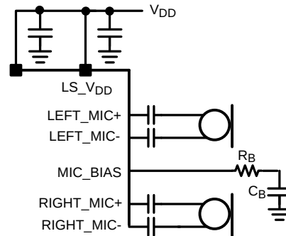
Figure 74. Schematic for MEMs Microphones
