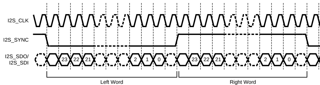
Figure 59. I²S Serial Data Format (24 bit example)
