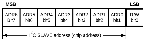
Figure 50. I²C Chip Address
