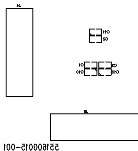
Figure 71. Bottom Silkscreen Layer
