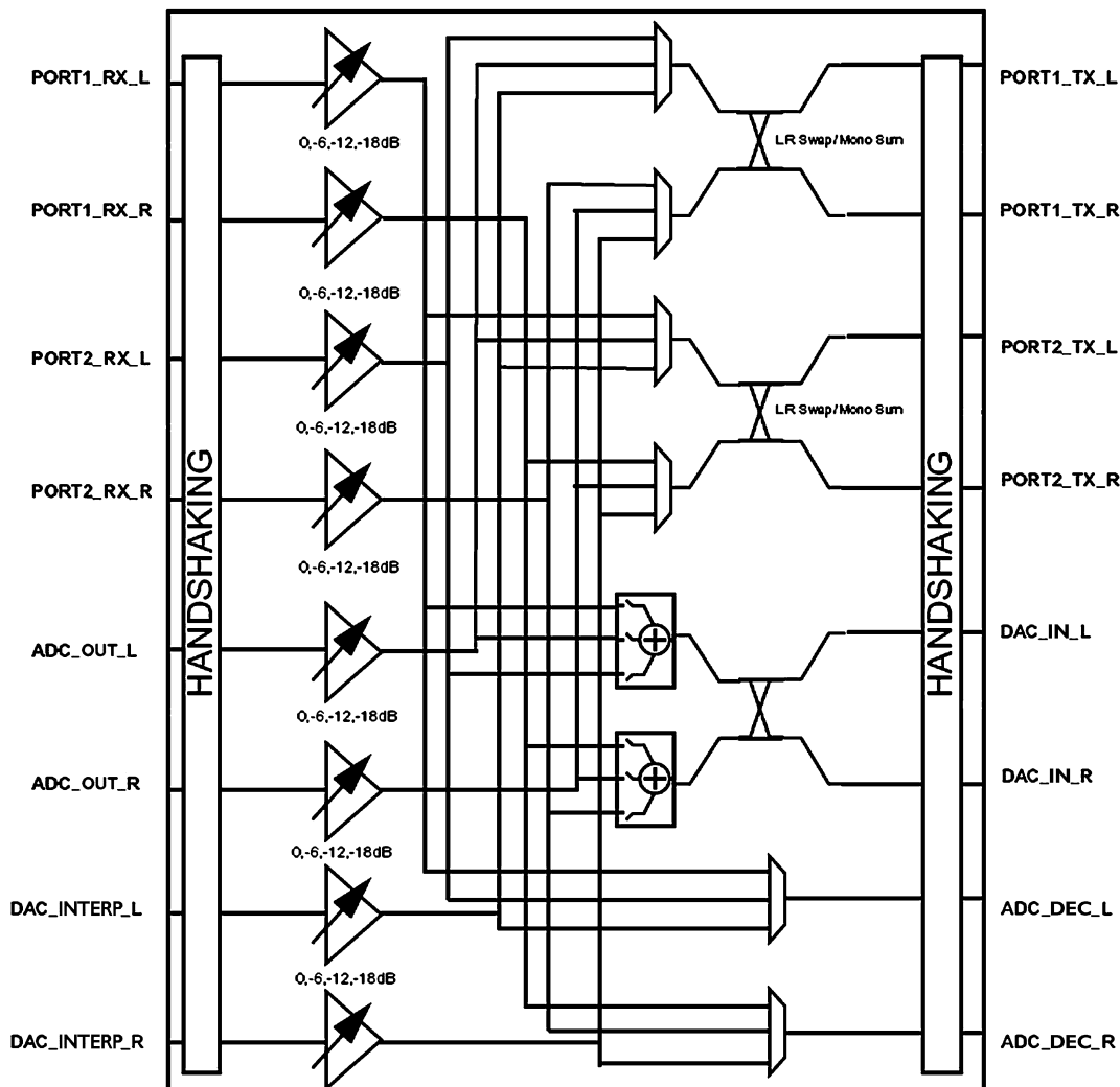
Figure 58. Digital Mixer
