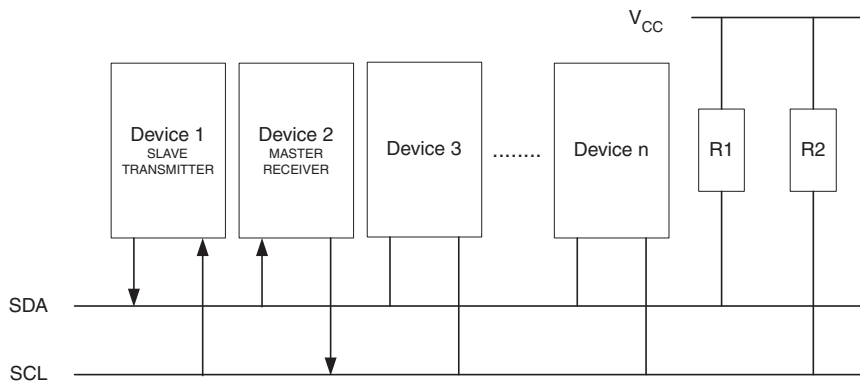
Figure 19-17. Data Transfer in Slave Transmitter Mode
