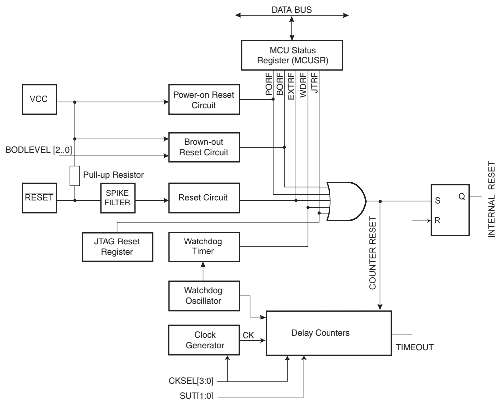
Figure 9-1. Reset Logic
