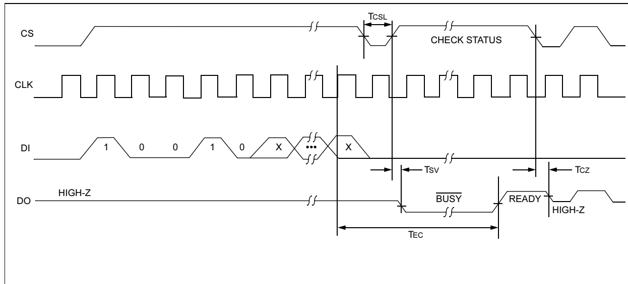
FIGURE 2-2: ERAL TIMING
