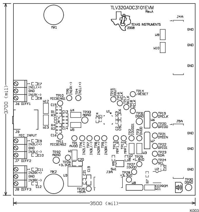
Figure 22. Top Overlay
