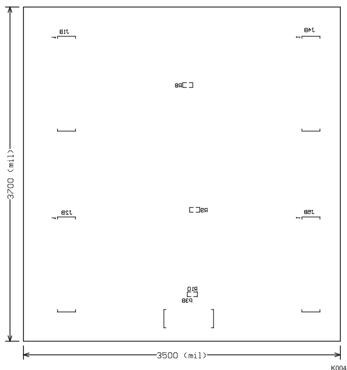
Figure 23. Bottom Overlay
