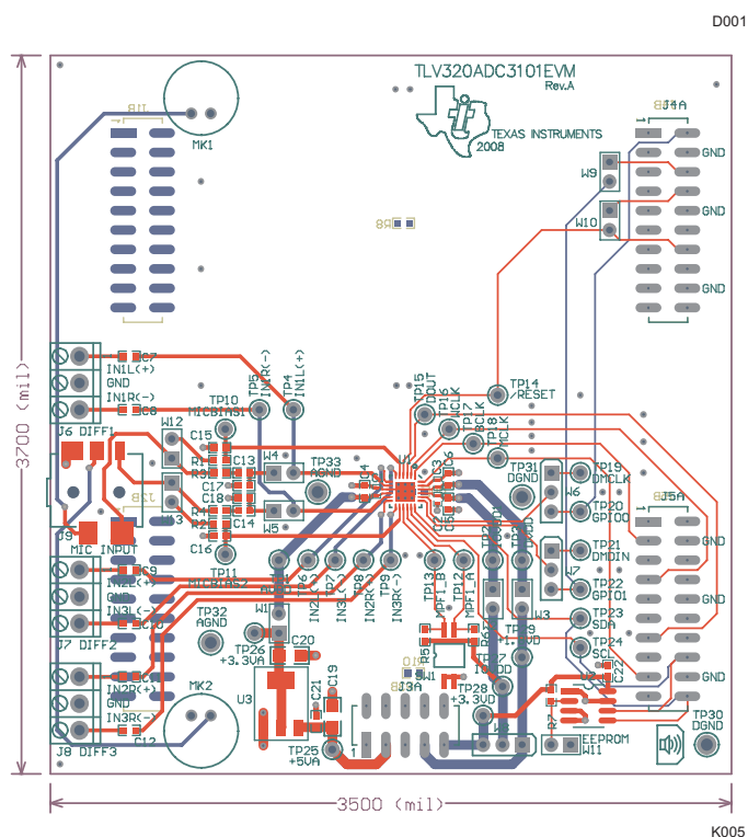
Figure 25. Composite
