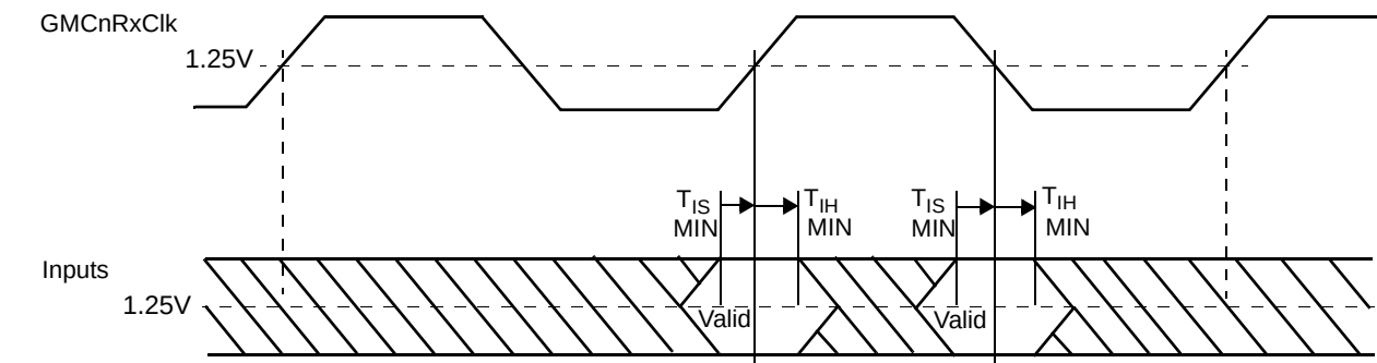
Figure 6. Input Setup and Hold Timing Waveform for RGMII Signals
