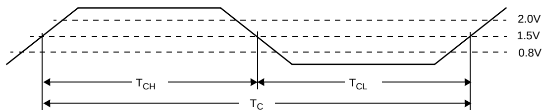
Figure 3. Clocking Waveform
