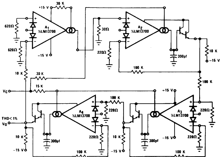
FIGURE 17. Sinusoidal VCO
