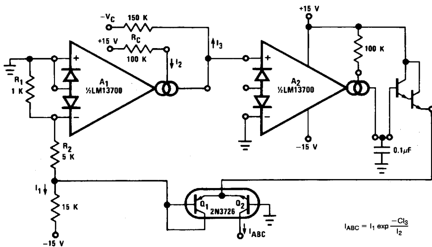
FIGURE 30. Logarithmic Current Source
