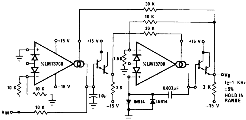
FIGURE 21. Phase Lock Loop
