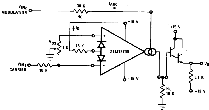
FIGURE 5. Amplitude Modulator
