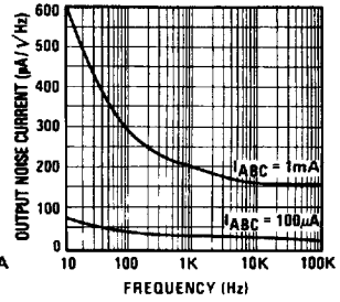
Output Noise vs Frequency
