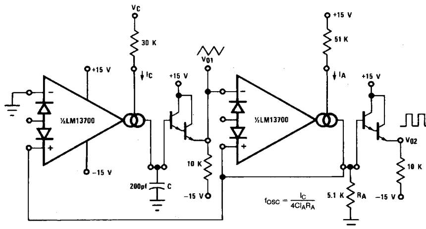
FIGURE 15. Triangular/Square-Wave VCO
