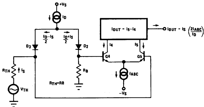
FIGURE 3. Equivalent VCA Input Circuit
