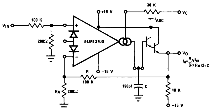
FIGURE 11. Voltage Controlled Low-Pass Filter
