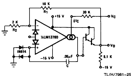
FIGURE 18. Single Amplifier VCO
