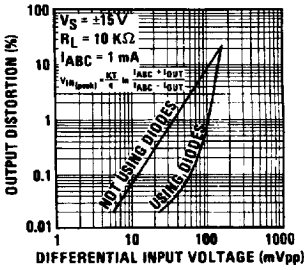
Distortion vs Differential Input Voltage
