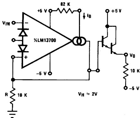
FIGURE 22. Schmitt Trigger
