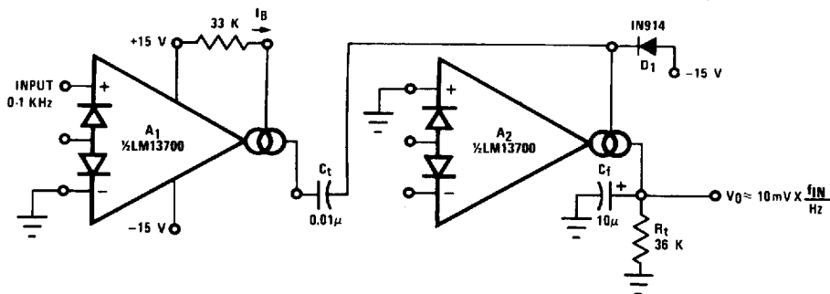
FIGURE 23. Tachometer
