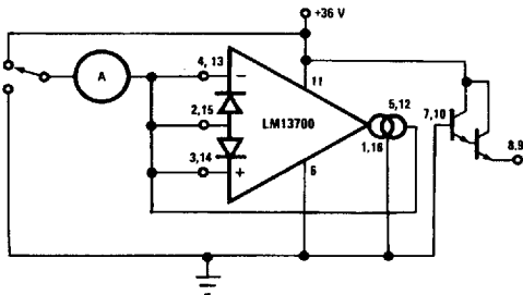
Leakage Current Test Circuit
