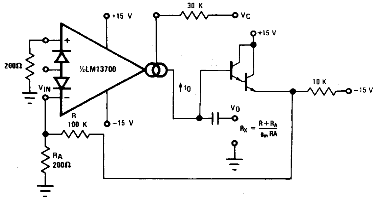
FIGURE 8. Voltage Controlled Resistor, Single-Ended
