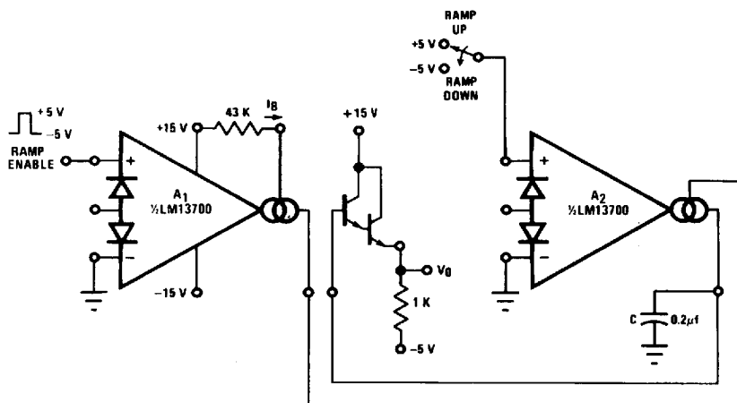
FIGURE 26. Ramp and Hold
