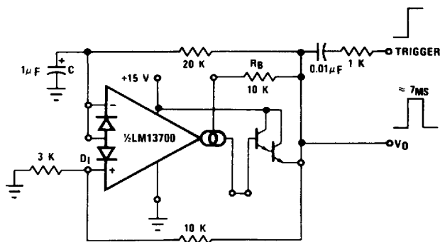
FIGURE 19. Zero Stand-By Power Timer
