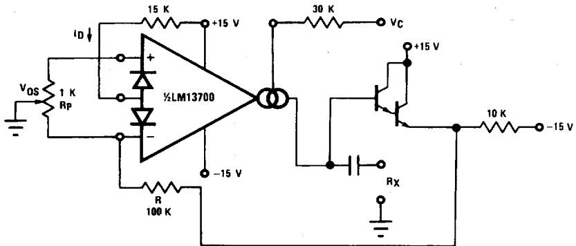
FIGURE 9. Voltage Controlled Resistor with Linearizing Diodes
