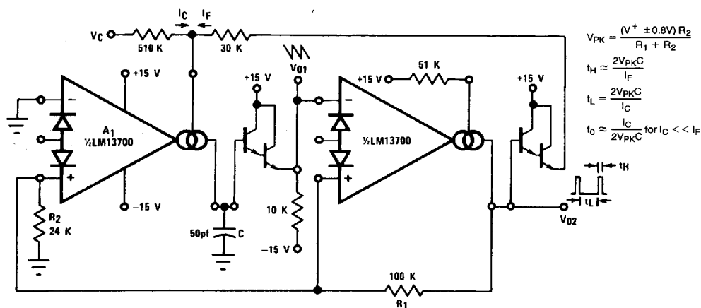
FIGURE 16. Ramp/Pulse VCO
