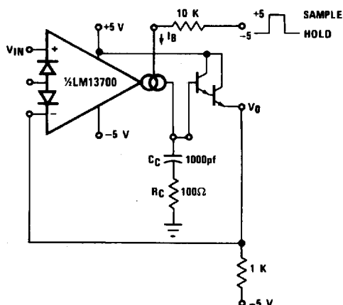
FIGURE 25. Sample-Hold Circuit
