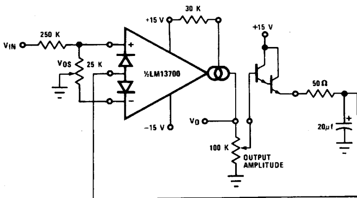
FIGURE 7. AGC Amplifier
