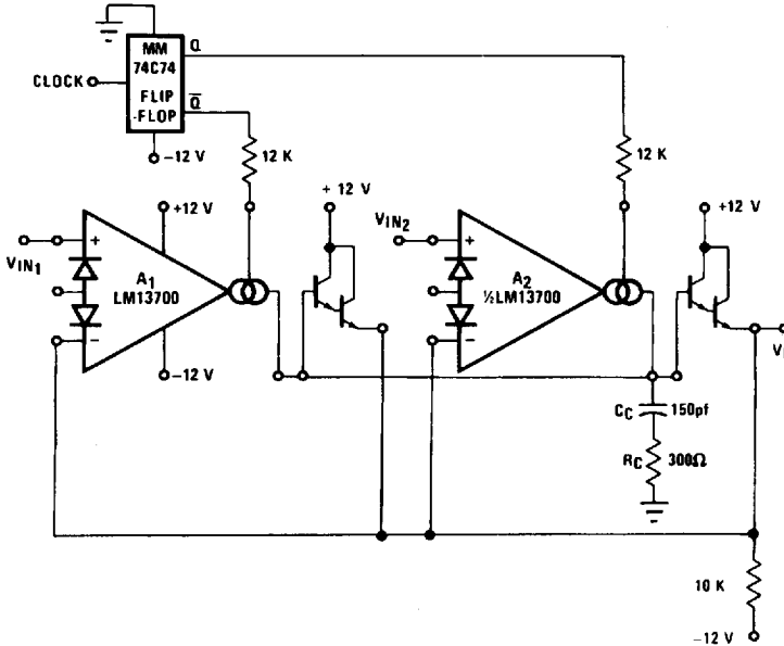
FIGURE 20. Multiplexer
