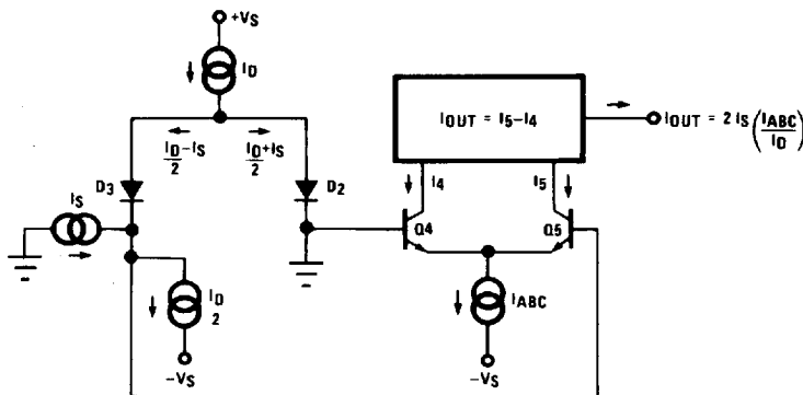
FIGURE 1. Linearizing Diodes
