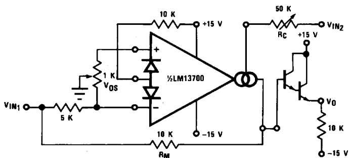
FIGURE 6. Four-Quadrant Multiplier
