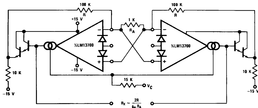
FIGURE 10. Floating Voltage Controlled Resistor
