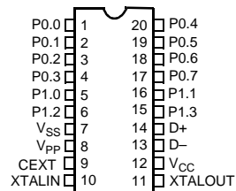
20-pin DIP/SOIC
