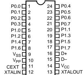
24-pin SOIC/QSOP
