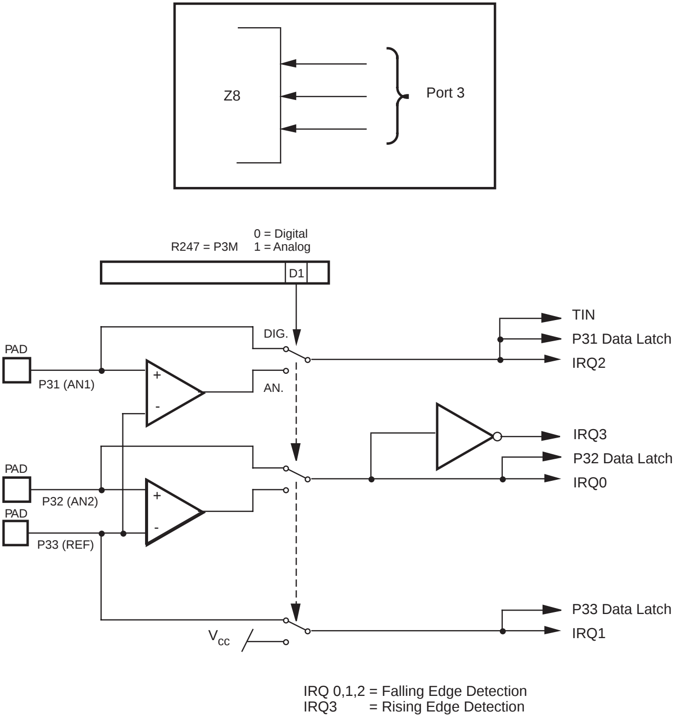
Figure 9. Port 3 Configuration
