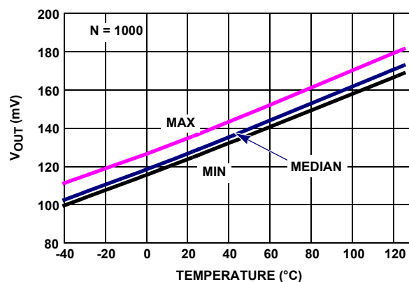
FIGURE 32. EL8173 V_{OUT} LOW vs TEMPERATURE, R_L = 1k , V_+ = \pm 2.5V
