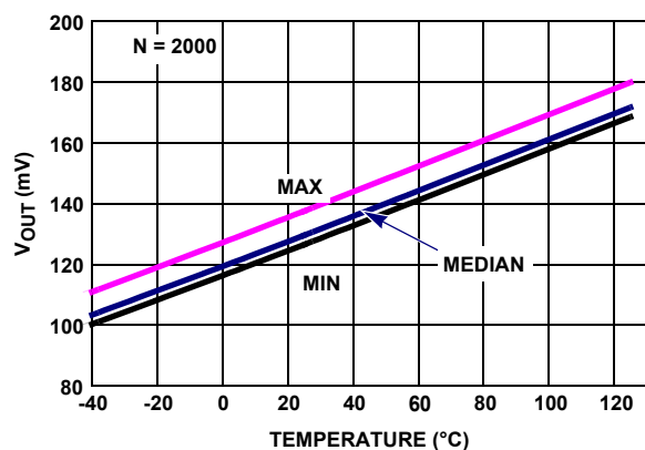
FIGURE 31. EL8170 V_{OUT} LOW vs TEMPERATURE, R_L = 1k , V_+ = \pm 2.5V
