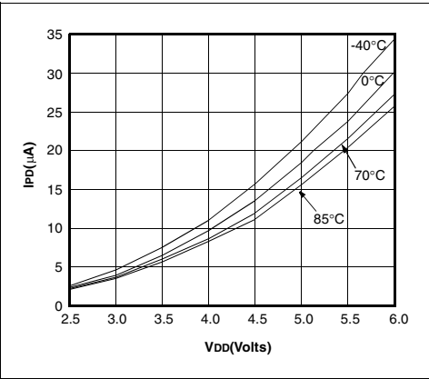
FIGURE 23-4: MAXIMUM I_{PD} vs. V_{DD} (WDT ENABLED, RC MODE)
