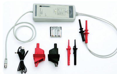
N2891A 70 MHz high voltage differential probe
