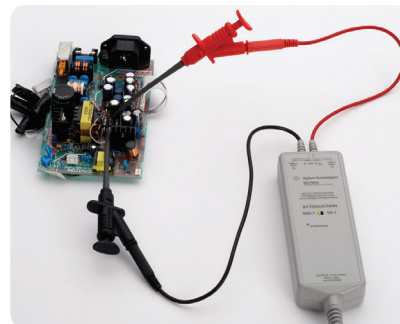
N2790A measuring a power supply signal
