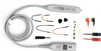
N2819A 800-MHz, 15-V differential probe with AutoProbe interface
