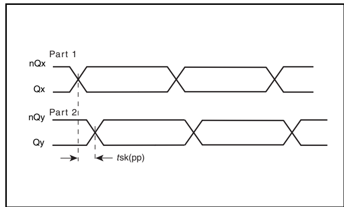
Part-to-Part Skew
