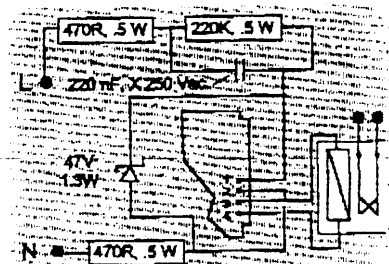
Capacitor PSU
