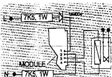
Two Resistor PSU - gives Optimum EMC Performance
