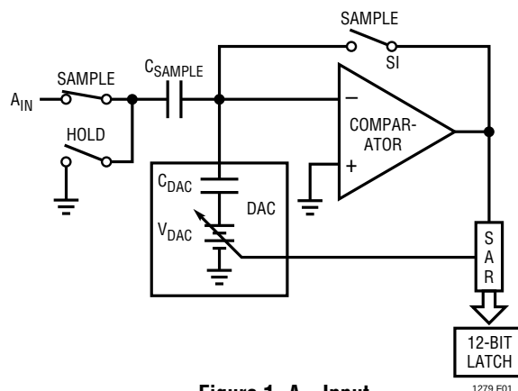
Figure 1. A_{IN} Input
