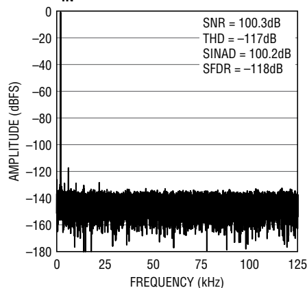
32k Point FFT f_s = 250\text{ksps} , f_{IN} = 2\text{kHz}
