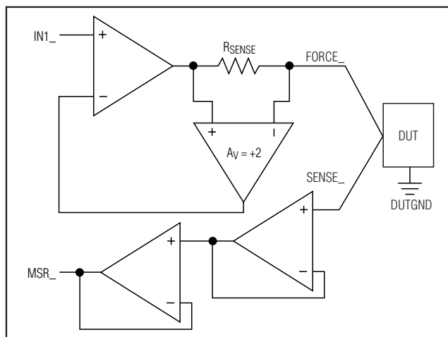
Figure 7. Force-Current/Measure-Voltage Functional Diagram
