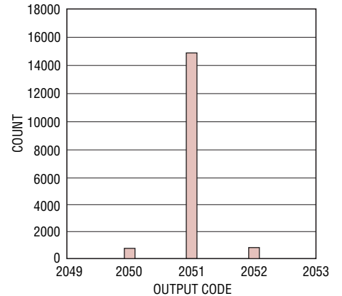
LTC2170-12: Shorted Input Histogram
